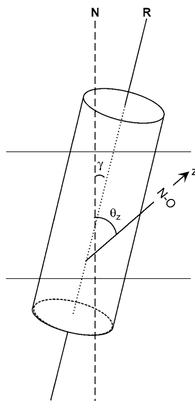
FIGURE 6 Orientation of TOAC-labeled alamethicin in a lipid membrane. The principal molecular diffusion axis, R , is inclined at instantaneous angle \gamma to the membrane normal N . The nitroxide z axis is oriented at constant angle \theta_z to R . The experimental order parameter, S_{zz} , of the nitroxide z axis is given by Eq. 6, where, for axial symmetry, \langle P_2(\cos\gamma) \rangle is the order parameter of the alamethicin diffusion axis.
